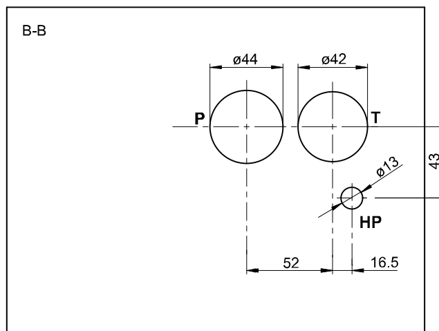
Pipe-mounting connection – see Figure B-B
