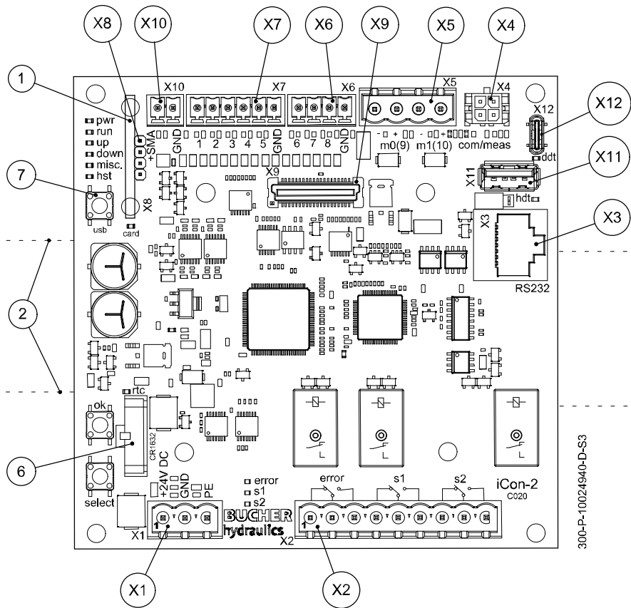
Control card iCon-2 – basic board
